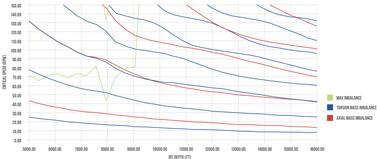
FIGURE 3: VARIATION OF CRITICAL RPM OVER DEPTH ILLUSTRATES OPTIMAL RPM TO REDUCE DOWNHOLE TOOL FAILURES
