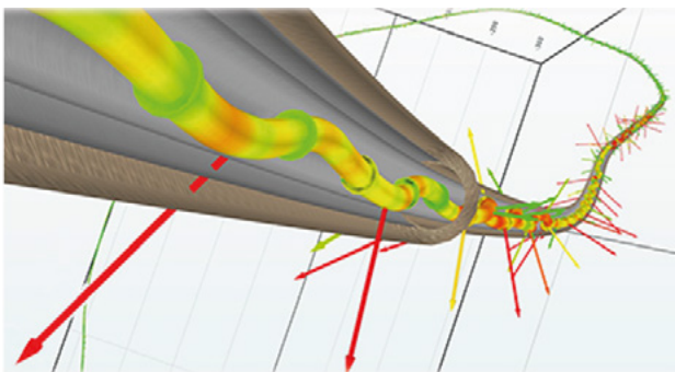
FIGURE 1: ADVANCED 3D VIEWER: HIGH LEVEL OF BUCKLING ALONG LANDING STRING WHILE RIH WITH LINER IN 3D DEEPWATER WELL
