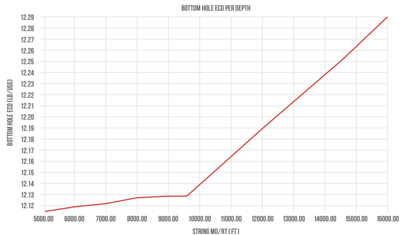
FIGURE 2: EVOLUTION OF BOTTOM-HOLE ECD FOR MULTIPLE BIT DEPTHS
